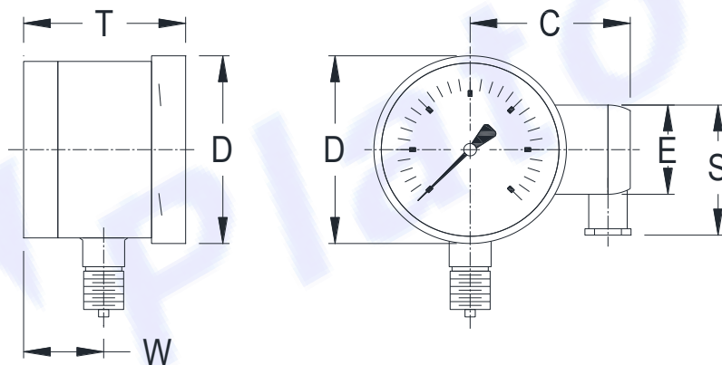
A (直立式)
