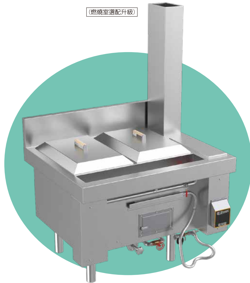
品名：雙口腸粉爐(右煙囪) 尺寸：W1100xD900xH800/1000(mm)
