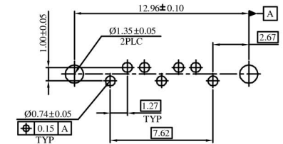
RECOMMEND PCB LAYOUT PCB TOLERANCE: ±0.05
