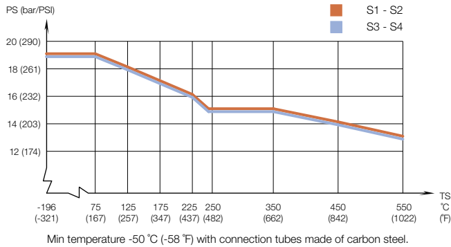
AlfaNova HP 400 – PED approval pressure/temperature graph*
