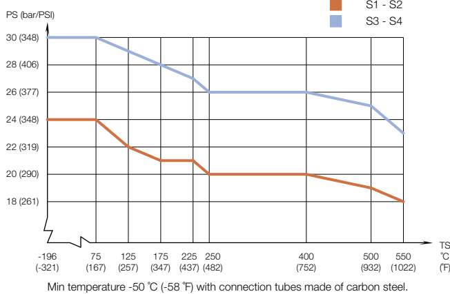
AlfaNova HP 400 – PED approval pressure/temperature graph*
