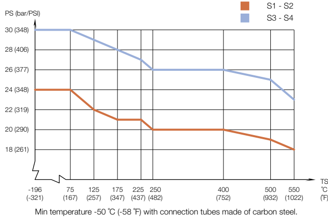
AlfaNova HP 400 – PED approval pressure/temperature graph*
