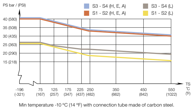
AlfaNova HP 76 – PED approval pressure/temperature graph*
