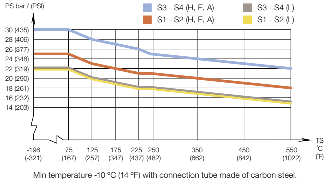
AlfaNova 76 – PED approval pressure/temperature graph*
