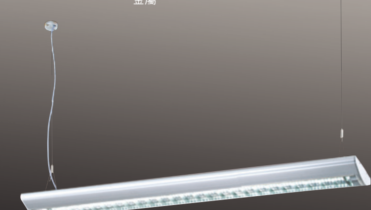
AL24808 14000 L1185mm W55mm H210mm 線長900mm 附T5 LED 18wx2 金屬、鋁格柵
