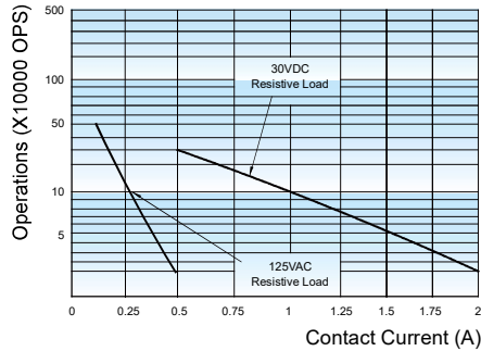
ENDURANCE CURVE
