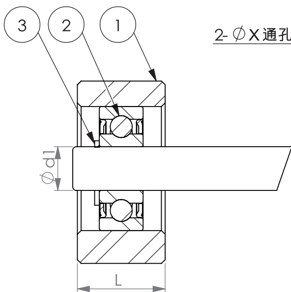
剖面圖 A-A Sectional View
