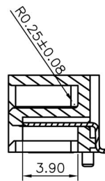
SECTION E-E
