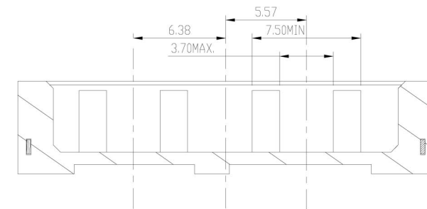
SECTION F-F
