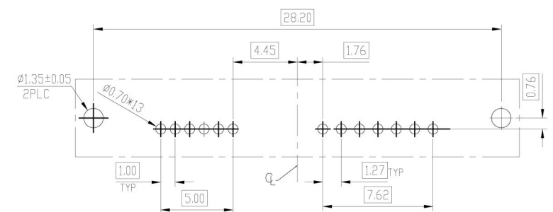
SECTION F-F
