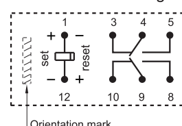
1 coil latching
