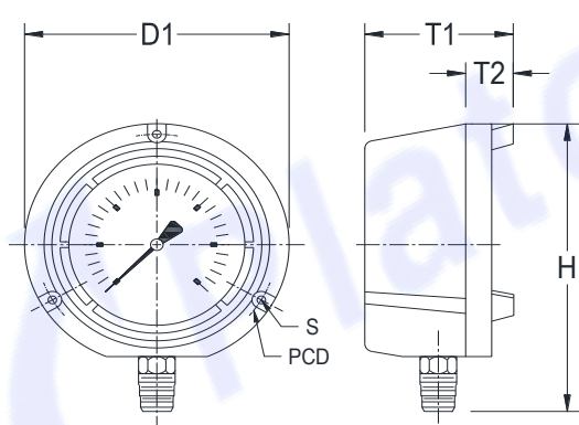
A (直立式)
