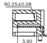
SECTION E-E
