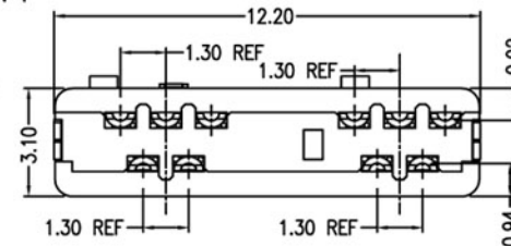
SEC B-B(PIN1, 5, 8 SECTION)
