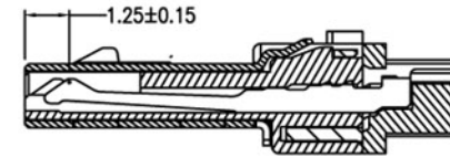
SEC B-B(PIN1, 5, 8 SECTION)
