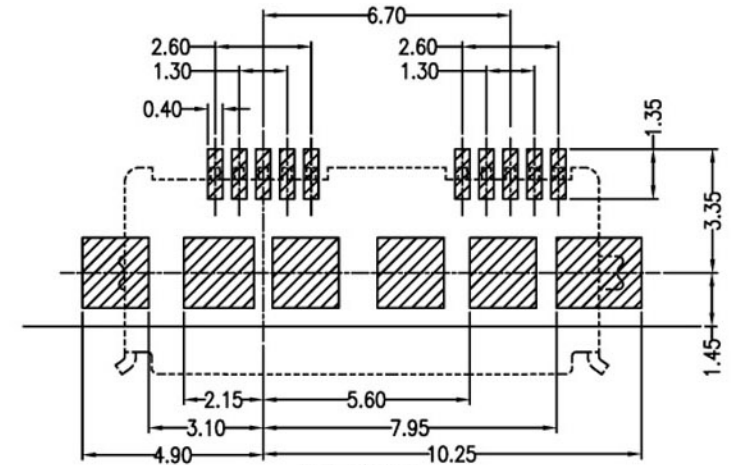
PCB LAYOUT COMPONENT SIDE TOLERANCE:±0.05
