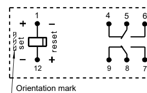
1 coil latching
