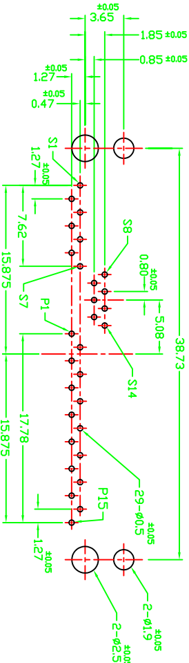
RECOMMENDED P.C.B. LAYOUT
