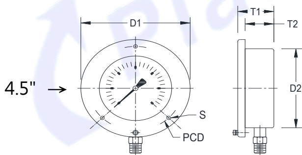
A (直立式)
