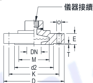
(1/2"~2"為膜片內藏式)
