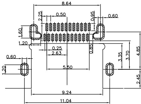
PCB LAYOUT (RECOMMENDED) (Tol: ±0.05)
