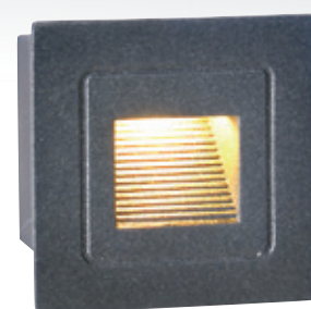
AL2672A 3000 L58mm W58mm H47mm 附LED 1wx1、暖白、全電壓 鋁合金壓鑄組裝成型、砂黑 噴砂玻璃、附ABS預埋盒 預埋盒：L45mm W45mm H46mm
