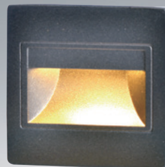
AL26724 3600 L94mm W94mm H49mm 附LED 3wx1、暖白、全電壓 鋁合金壓鑄組裝成型、砂黑 噴砂玻璃、附ABS預埋盒 預埋盒：L85mm W85mm H46mm
