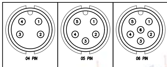
Pin Assignments(Front View)
