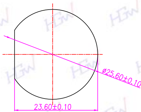
RECOMMEND PANEL HOLE
