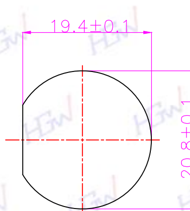
RECOMMEND PANEL CUT-OUT
