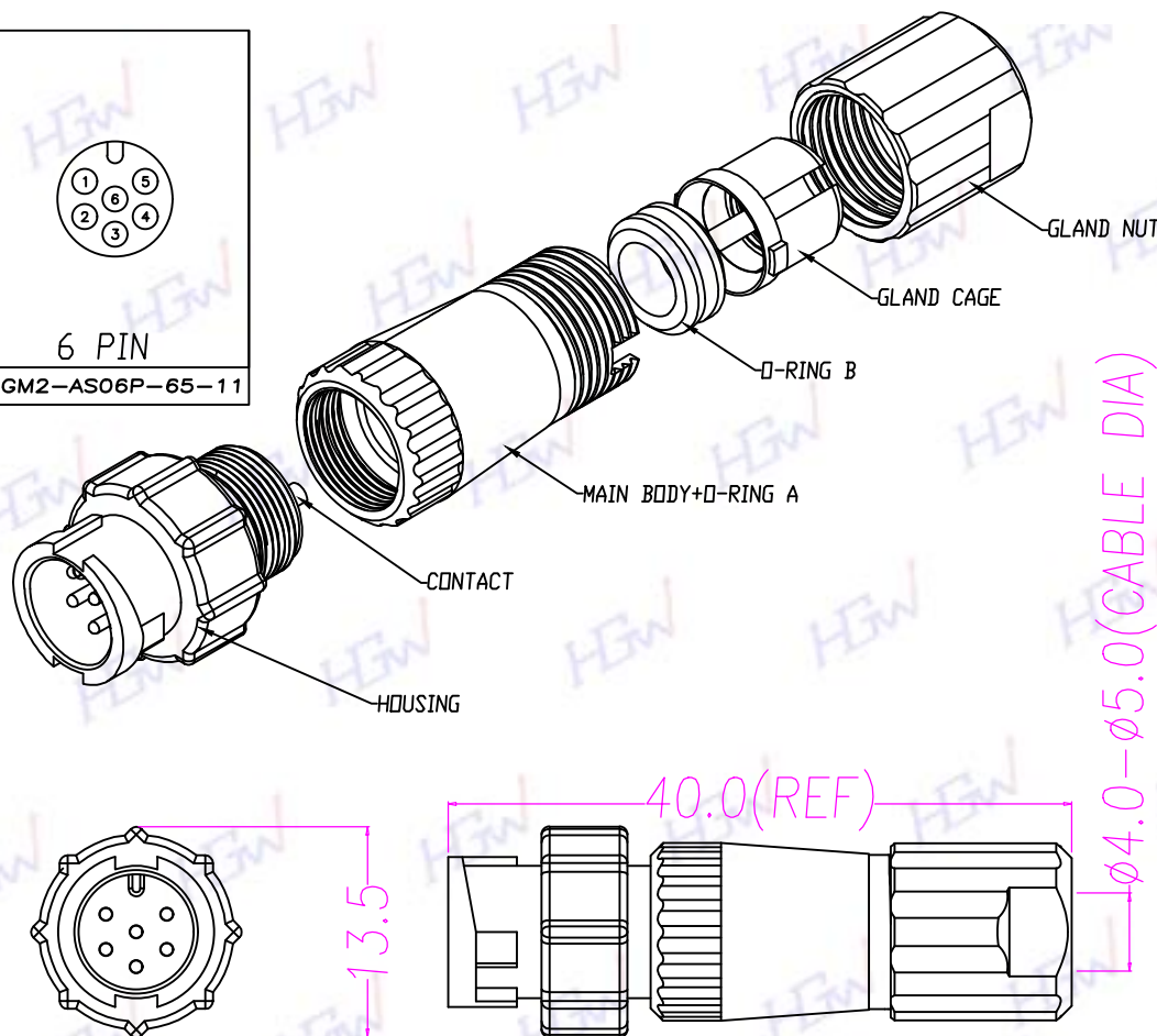
PIN ASSIGMENTS FRONT VIEW
