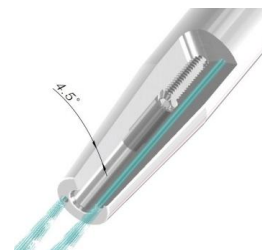
EZSB=4.5度斜角細型+止動螺絲 EZSB=4.5° Slim with back up screw EZSBKK=4.5度斜角鼻端出水細型附螺絲 EZSBKK=4.5° Slim with coolant through nose and with back up screw
