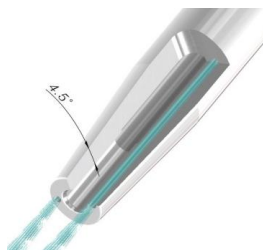
EZS=4.5度斜角細型 EZS=4.5° Slim EZSKK=4.5度斜角鼻端出水細型 EZSKK=4.5° Slim with coolant through nose
