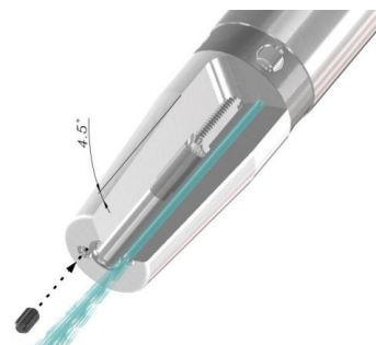
EZKK=4.5度斜角鼻端出水標準型 EZKK=4.5° regular with coolant through nose
