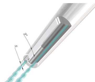
EZSRKK=3度斜角鼻端出水細型 EZSRKK=3° SlimRegular with coolant through nose
