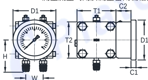
( 4" 不銹鋼差壓錶 ↑ )
