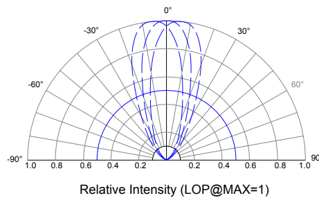
Beam Pattern
